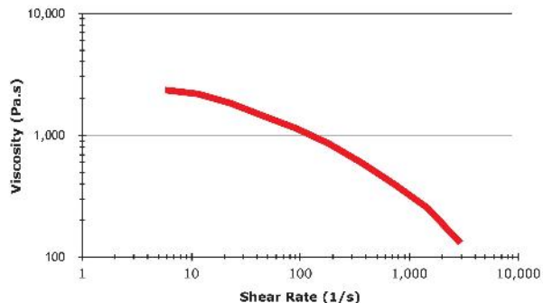
Shear-Viscosity @ 190 °C
